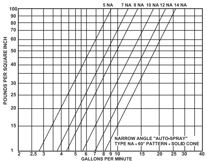
DISCHARGE CHARACTERISTICS
